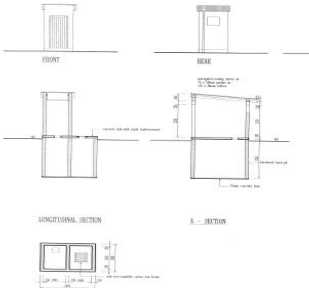
Figure 66 Concrete Lined Pit - Home Based Care Waste Disposal
