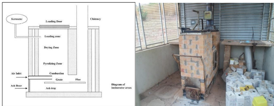
Figure 63 Incinerator Designs
